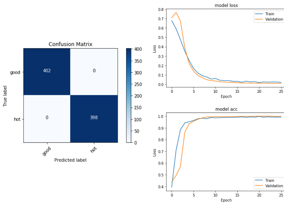
Figure 5.4: Confusion Matrix results and Learning curve for 5 \times 5 damaged area with on the random location for all trials
