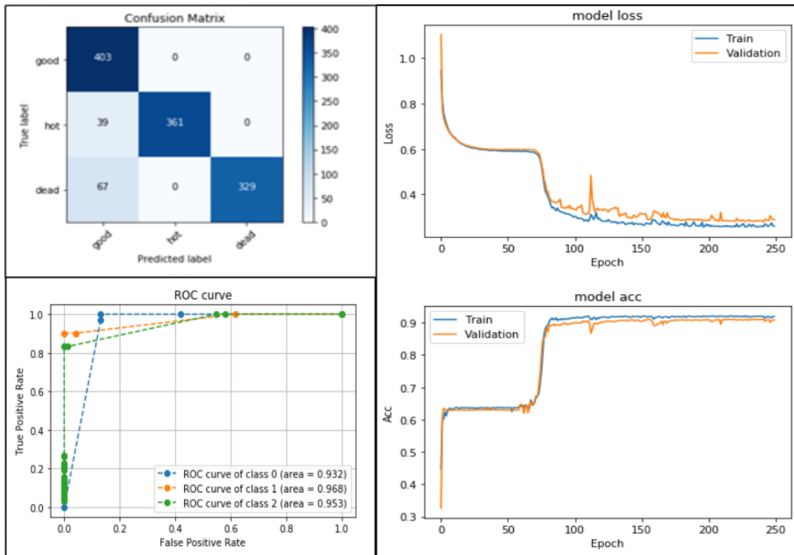
Figure 5.8: Three convolutional layers model results
