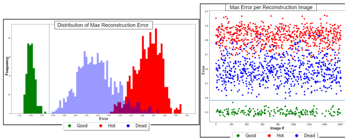
Figure 5.13: This histogram shows the distribution of error of the reconstruction and the dot plot on the right show the error of reconstruction of each image
