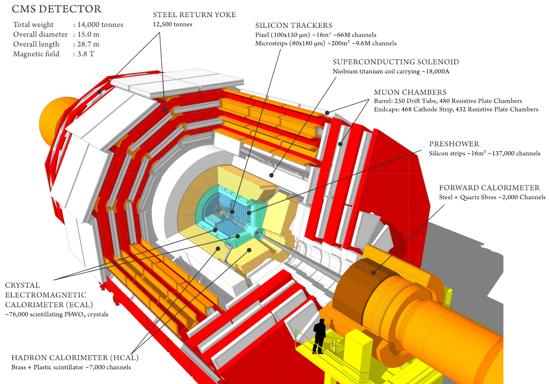
Figure 2.1: CMS Detector
