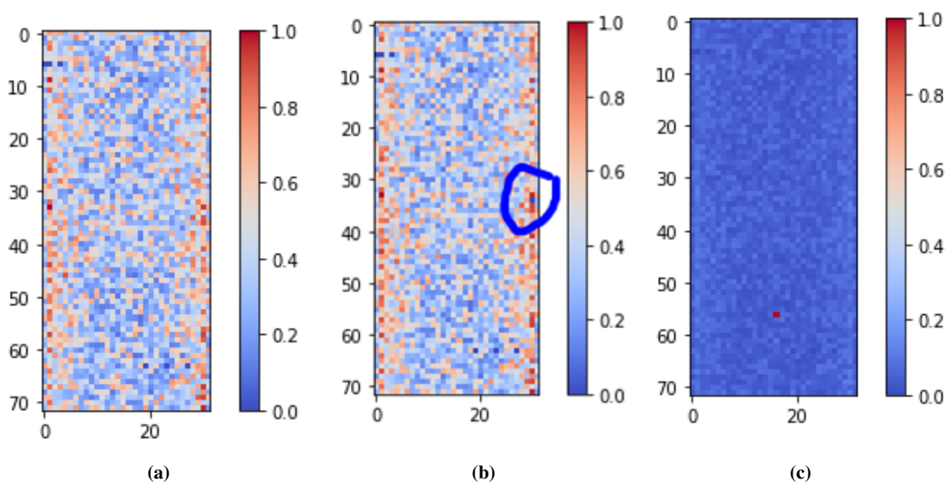
Figure 5.1: Occupancy Maps with 1 \times 1 bad regions. A) Good image B) Dead image C) Hot image
