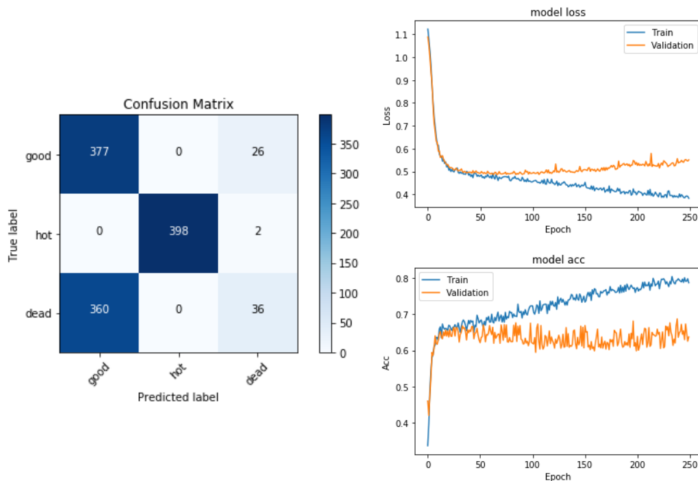
Figure 5.6: Confusion Matrix results and Learning curve for 1 \times 1 damaged area with random location for all trials
