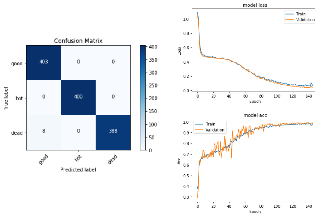
Figure 5.5: Confusion Matrix results and Learning curve for 5 \times 5 damaged area with an extra class to identify with random location for all trials
