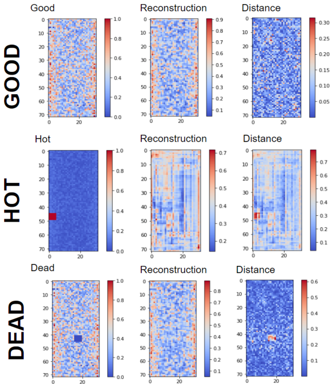
Figure 5.12: Inputs, Reconstruction and distance maps for the SSL model
